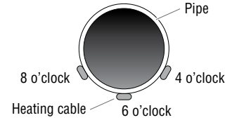
Heating Cable Position
